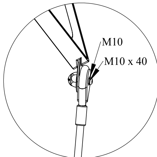
DETAIL E SCALE 1 : 5
